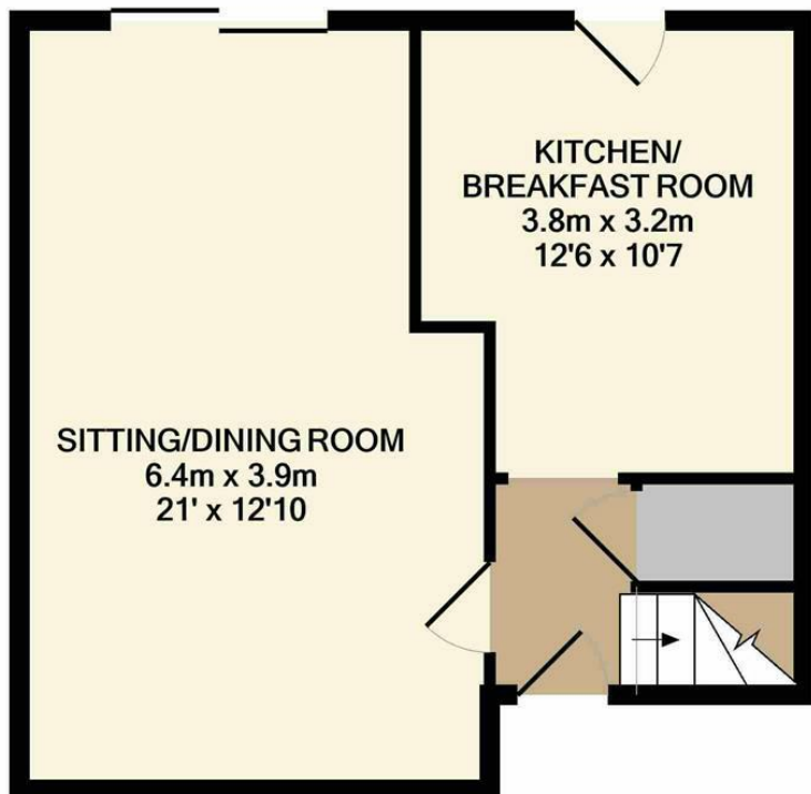
GROUND FLOOR APPROX. FLOOR AREA 39.7 SQ.M. (427 SQ.FT.)
